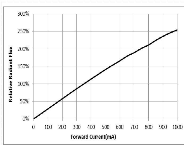
Fig 2. Forward Current vs. Relative Intensity, T_a = 25^\circ\text{C}
